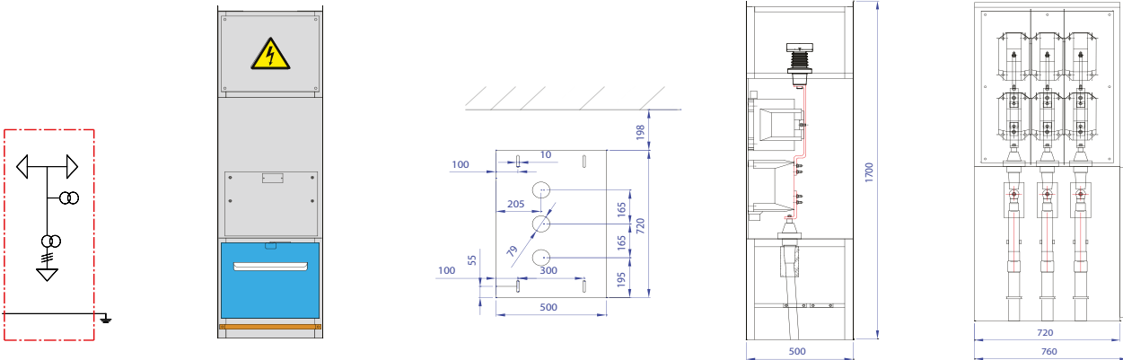
This setup: bottom in left or right out with busbar connection
